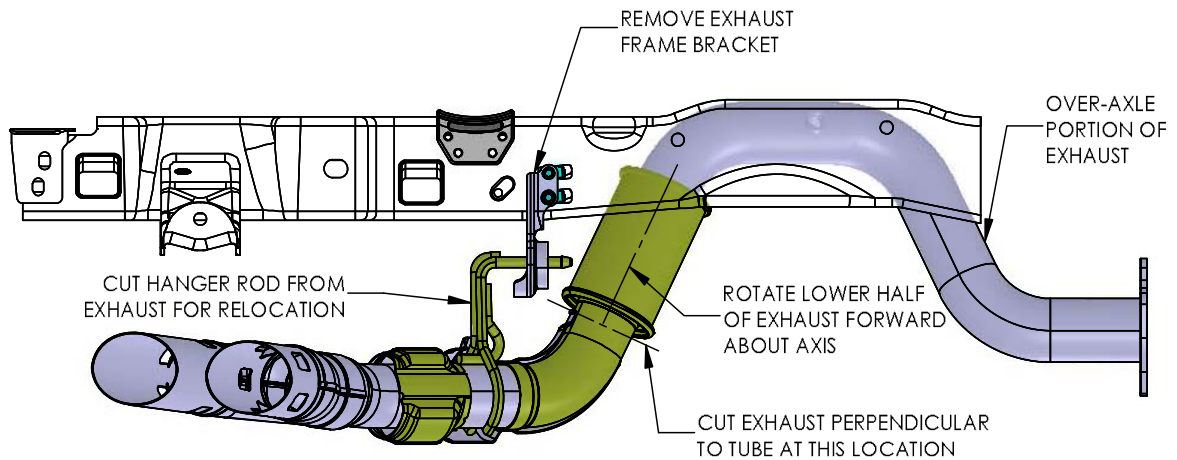
Figure 4.7.2.A F250/350 Diesel Exhaust Modifications
