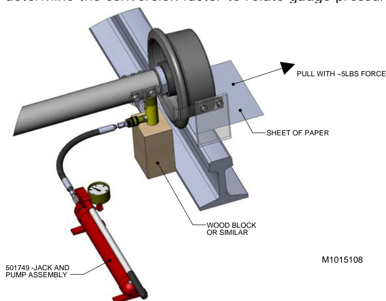
Figure 4.6.4. Checking rail wheel load
