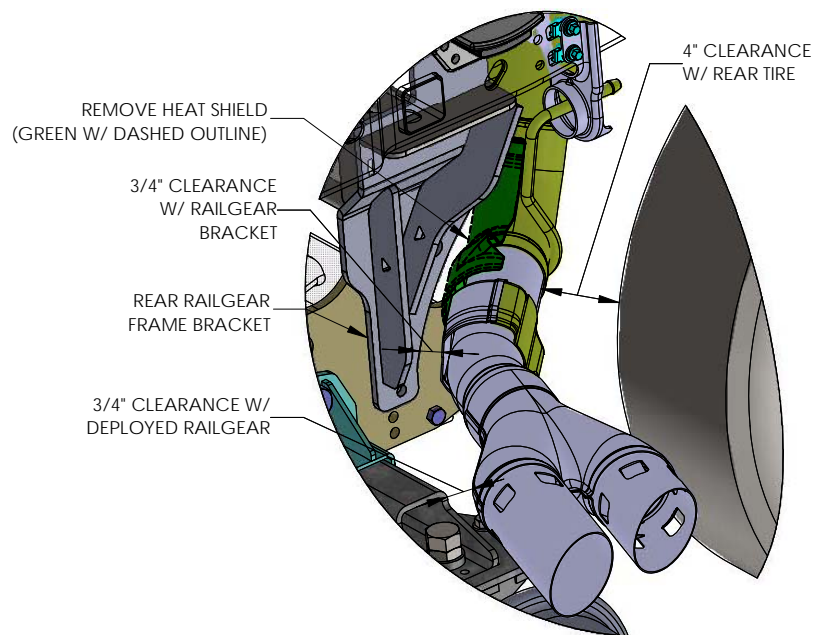
Figure 4.7.2.B F250/350 Diesel Exhaust Clearances
