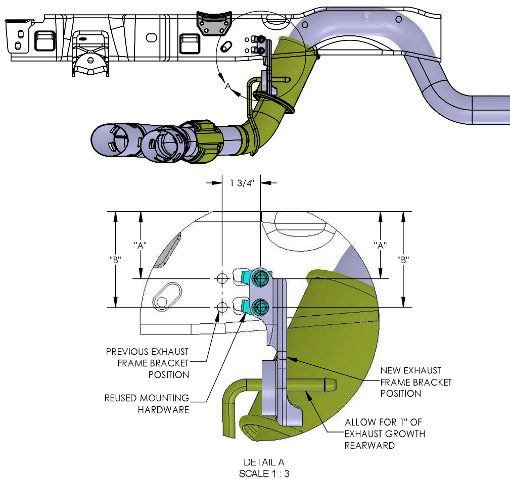
Figure 4.7.2.C F-250/350 Diesel Exhaust Hanger Modification
