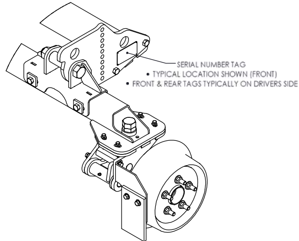
Figure 6.1.1 RW-1016 Typical Serial Number Locations
